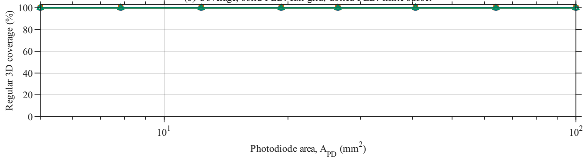
(b) Coverage; solid PEB: full grid, dotted PEB: finite subset
